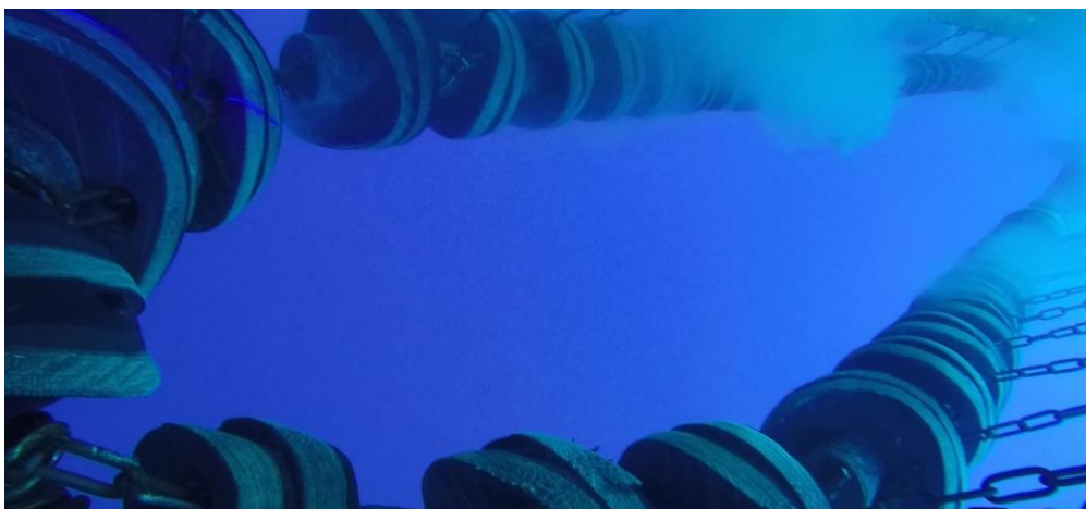
Fishing line before shooting trawl
